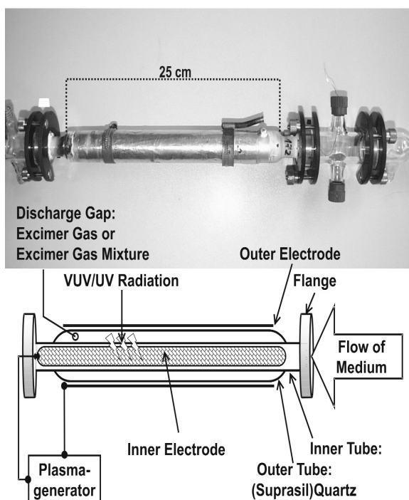
Figure 4: Schematic representation and photograph of an excilamp flow-through photoreactor (100 W – 1.5 kW) driven by DBDs, indicating the flow of the medium (gas or water)
