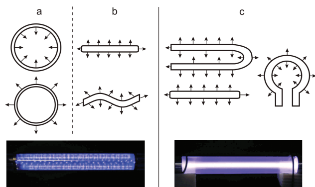
Figure 2. Geometry of barrier discharge (a, b) and capacitive discharge (c) excilamps: a – coaxial, b – planar or optional, c – cylindrical and its derivatives. The photographs demonstrate the typical view of discharges
