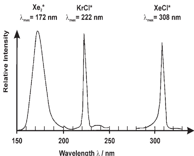
Figure 1. Emission spectra of DBD-driven \text{Xe}_2^* , \text{KrCl}^* and \text{XeCl}^* excilamps (c.f., Kogelschatz 2004).
