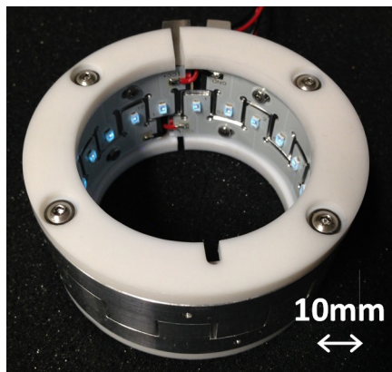
Figure 1. A ring-shaped UV LED apparatus (Oguma et al. 2016a)
